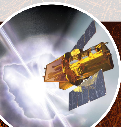
SWIFT
