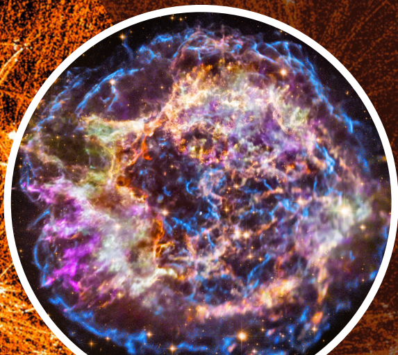
CHANDRA
